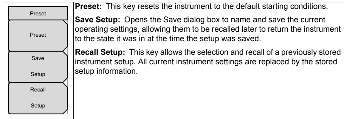
Figure 5-8. Preset Menu
