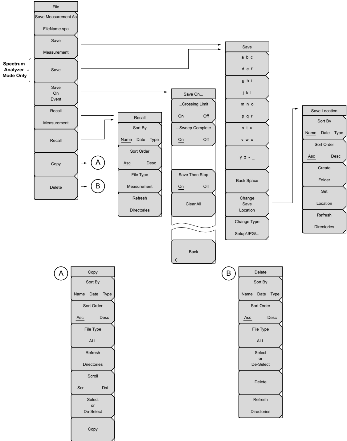
Figure 4-5. File Menu
