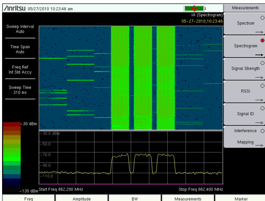
Figure 3-1. Spectrogram Example
